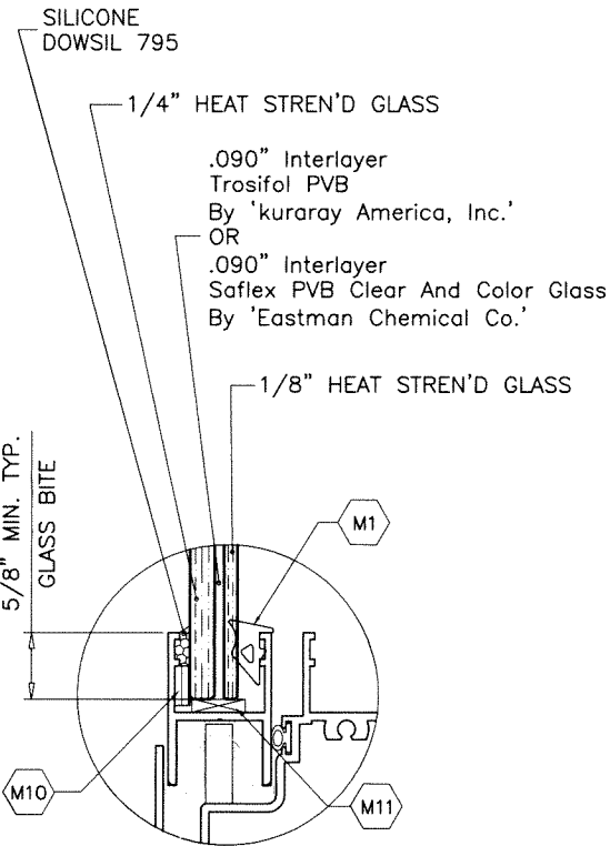
GLAZING DETAILS
